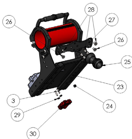
Exploded view of central and electronics units
